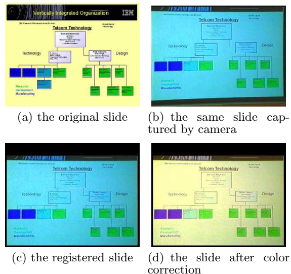
Figure 4: Color correction
